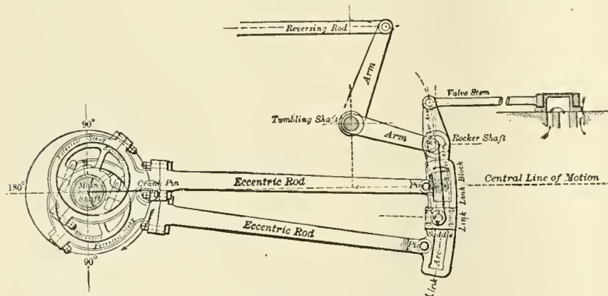
FIG. 2. INDIRECT VALVE MOTION.
